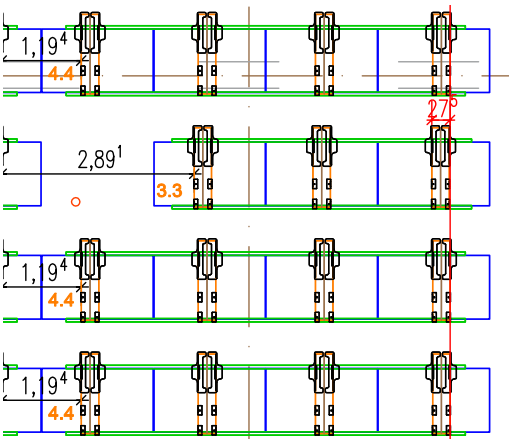
Computer-generated roof-specific PV module installation plan
